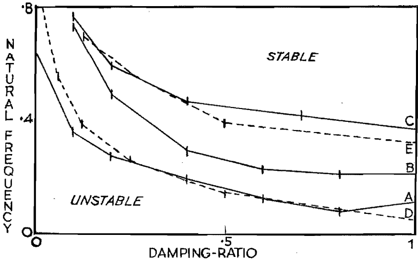
Fig. 5. — Stability boundaries for human and automatic control
