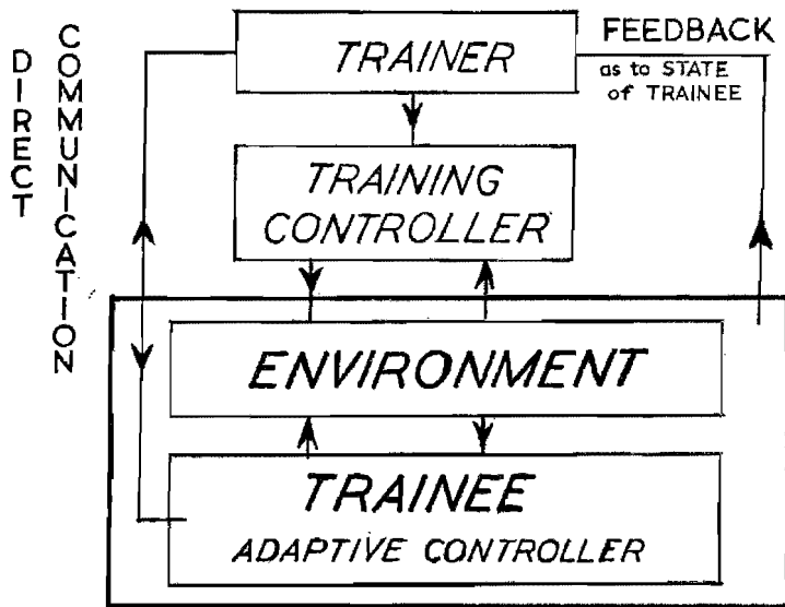
Fig. 2. — Feedback training system
